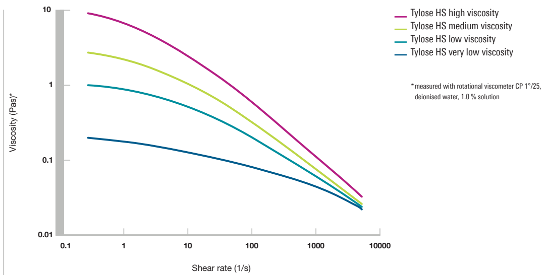
Pseudoplastic behaviour of Tylose
