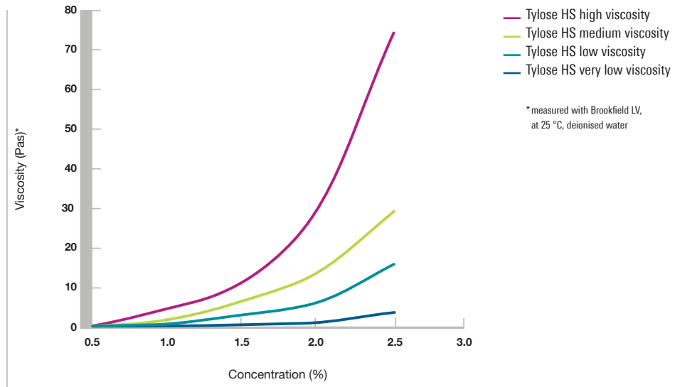
Influence of the concentration on the thickening effect of Tylose
